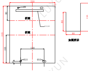
MEK挡水皮 1209000085
